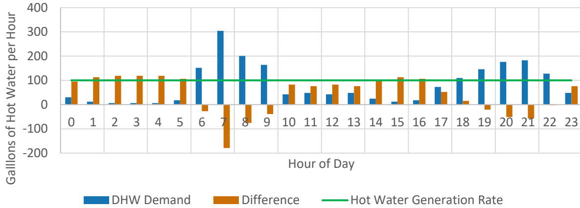
Figure 8. Hot water (HW) use, heating rate and difference throughout the day.
